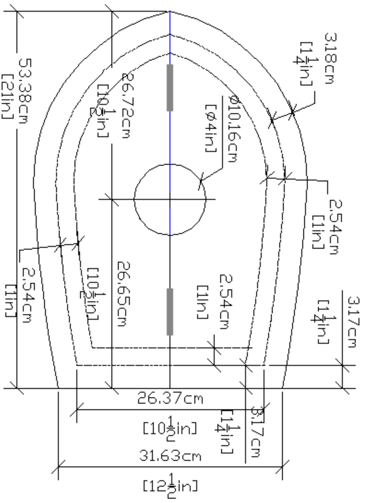
The Horizontal Plan for the Lid
